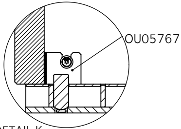
DETAIL K SCALE 1 : 5
