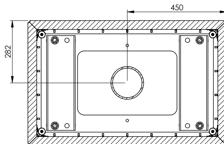
SECTION U-U SCALE 1 : 10
