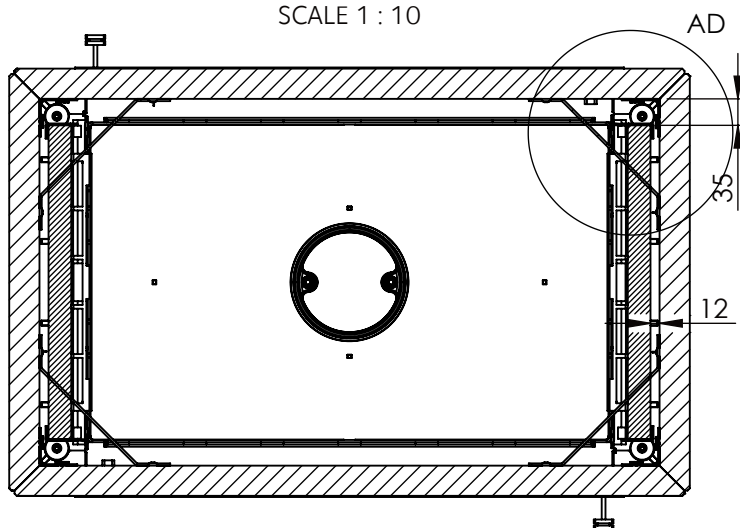
SECTION Y-Y SCALE 1 : 10
