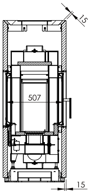
SECTION H-H SCALE 1 : 20
