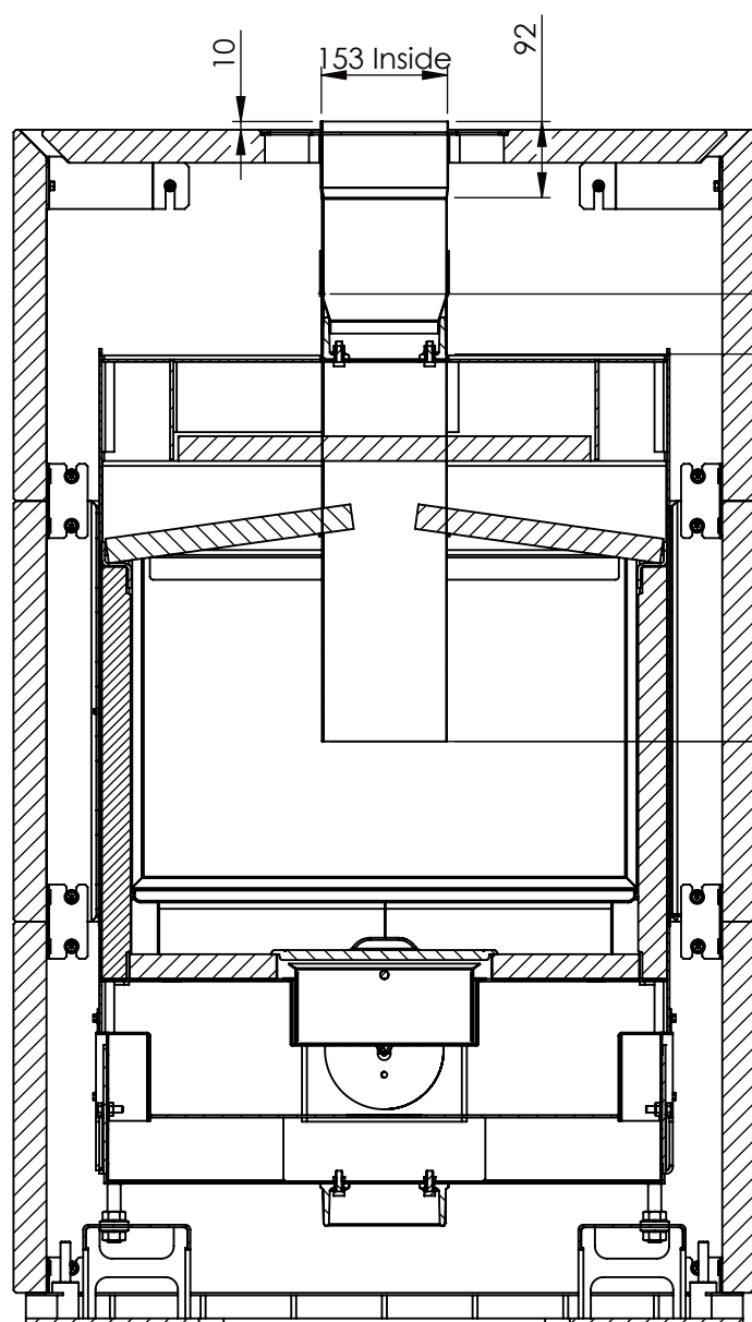
SECTION S-S SCALE 1 : 10
