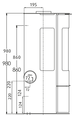
WESTFIRE.UNIQ.36 WESTFIRE.UNIQ.37 VEKT: 90 KG
