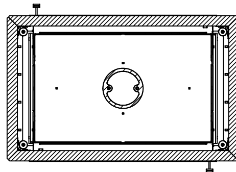
SECTION C-C SCALE 1 : 15
