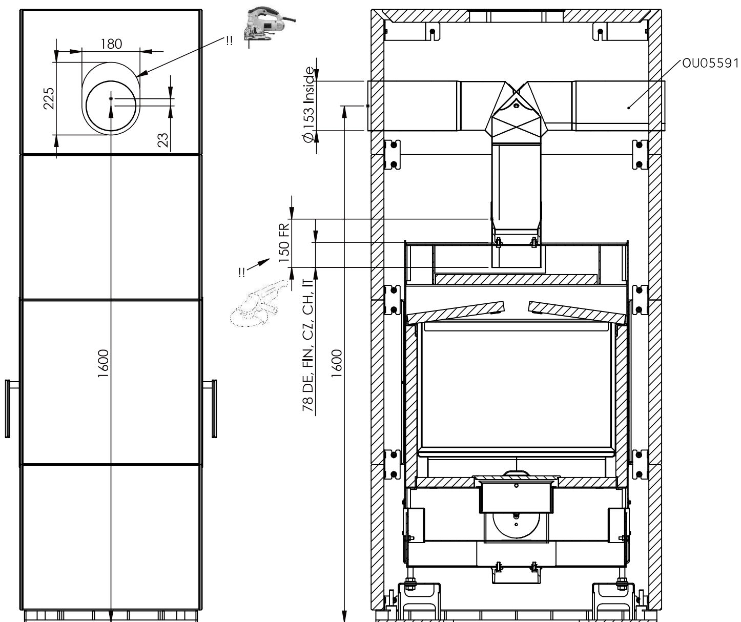
SECTION U-U SCALE 1 : 12
