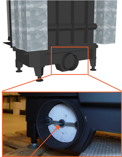
Hylse for "Large Room Heater"
