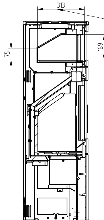
SECTION B-B
