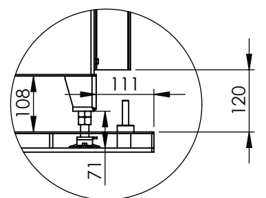
DETAIL J SCALE 1 : 10
