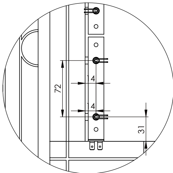
DETAIL R SCALE 1 : 3
