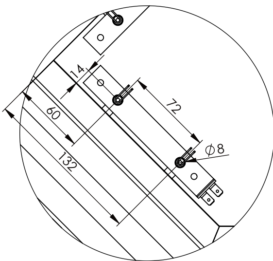
DETAIL A SCALE 1 : 3
