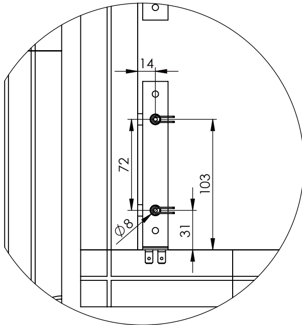
DETAIL B SCALE 1 : 3
