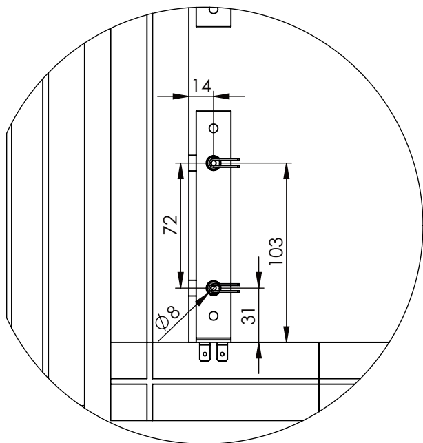
DETAIL M SCALE 1 : 3
